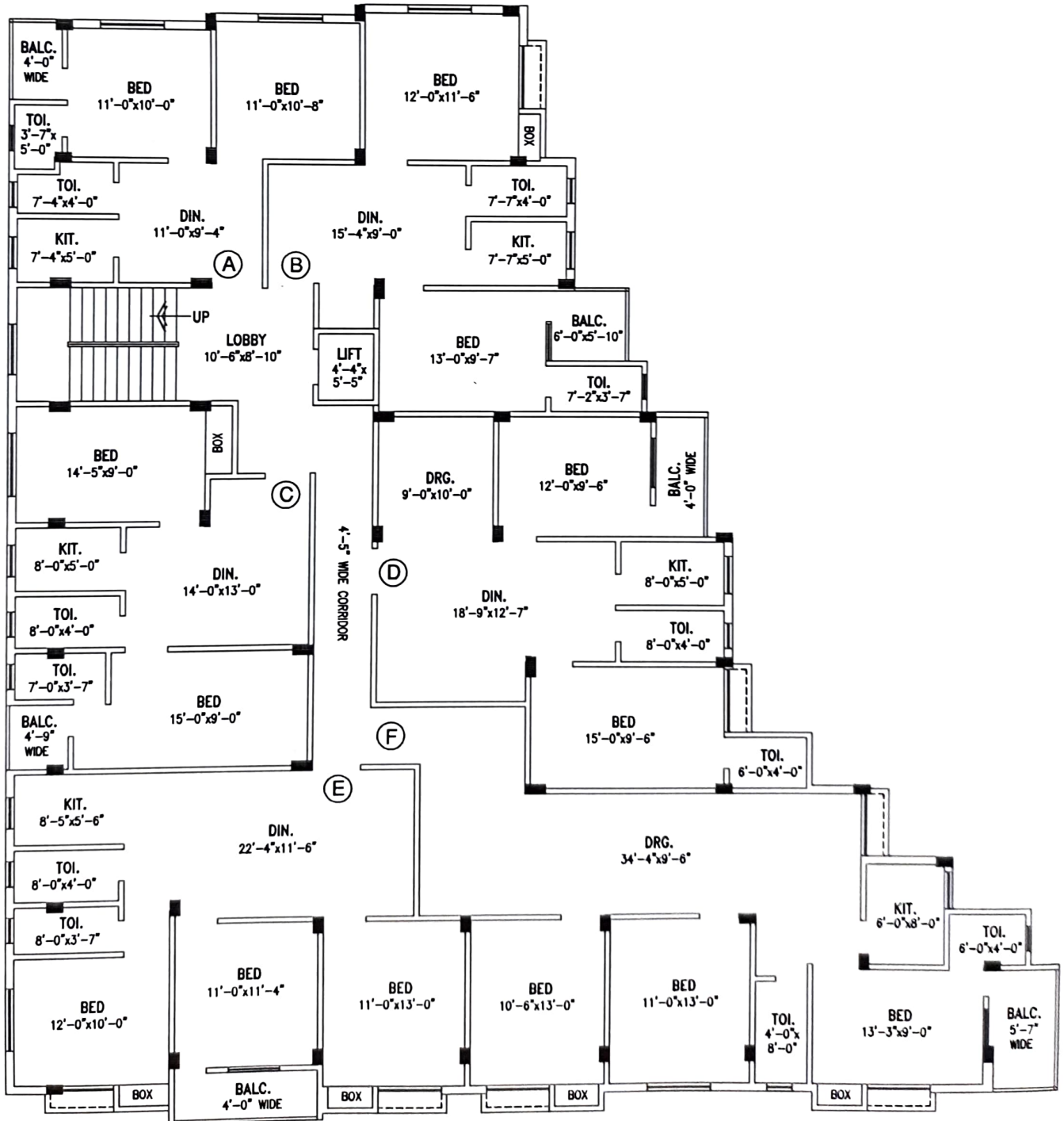
1ST.-4TH. FLOOR PLAN
