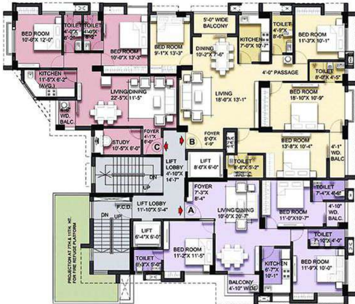
FLOOR PLAN
