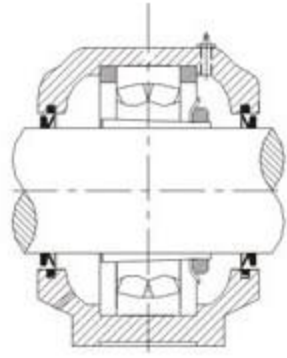
TA Type Design V-Ring with GI Lip Waser
