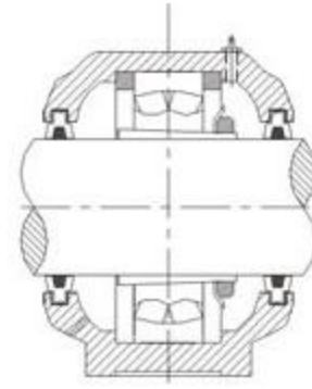
TC Type Design Felt Collar
