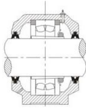
TG Type Design Double Lip Seal
